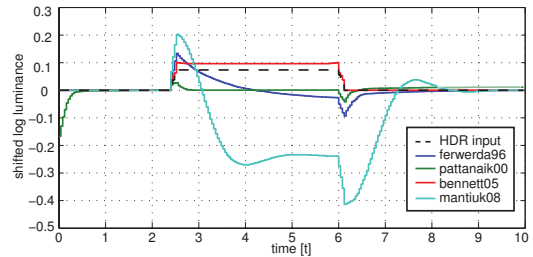
Figure 1: Left: The HDR-video sequences used in our evaluation exhibit strong local contrast changes, rapid variations in local and global intensity as well as spatio-temporal variations. Right: the plot illustrates how different a set of representative TMOs from our evaluation, see legend, responds to the same HDR input. The plot shows the log luminance of the temporal variation of a pixel under the green square as the light bulbs are turned on and off. Note that the plots are, for presentation purposes, shifted along the y-axis to start at the same value.
